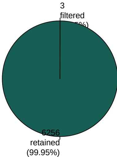
consensusPeaks
