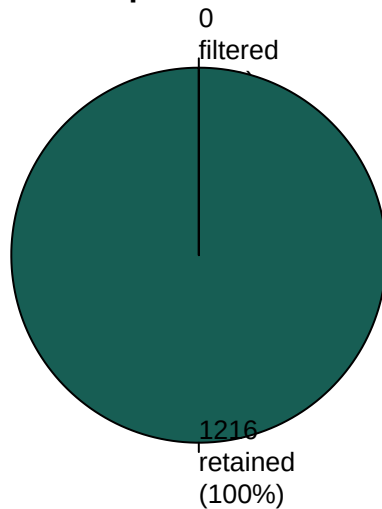
promoter
